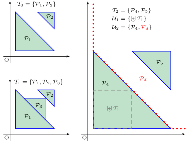
Fig. 7. The condition \#\mathcal{U}_1 > 1 is needed to obtain a proper widening.
