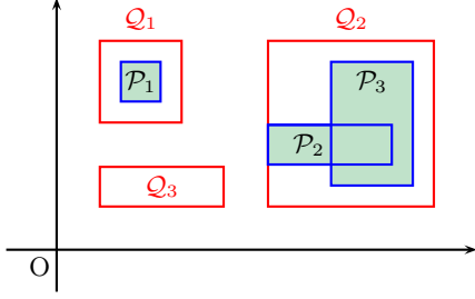
Fig. 1. The collection of \mathcal{Q}_i approximates the collection of \mathcal{P}_i .
