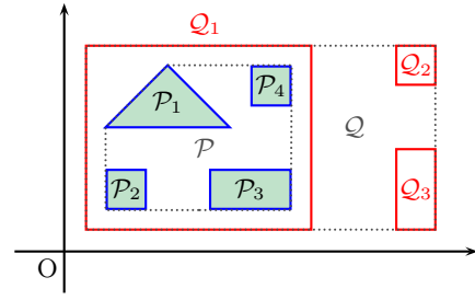
Fig. 3. The lgo relation on collections of polyhedra.
